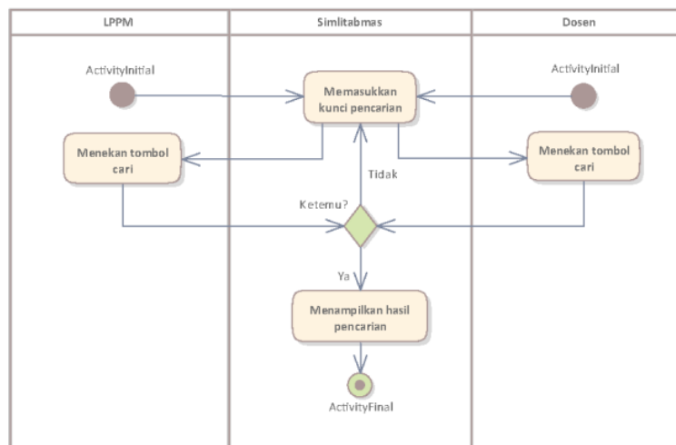
Gambar 5. Activity Diagram Cari Data
