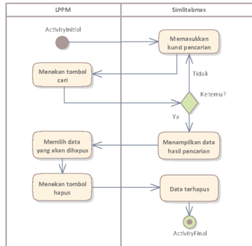
Gambar 7. Activity Diagram Hapus Data
