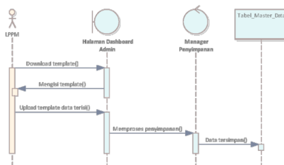
Gambar 10. Sequence Diagram Input Data
