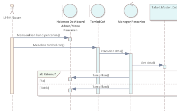
Gambar 11. Sequence Diagram Cari Data
