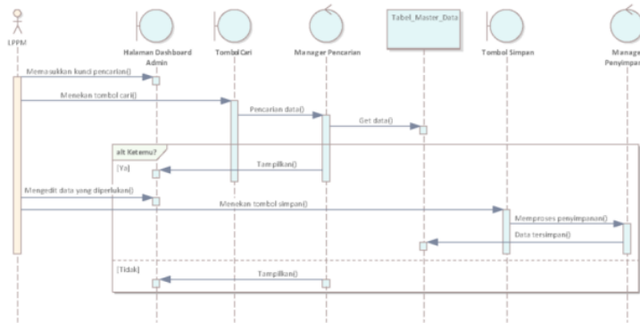
Gambar 12. Sequence Diagram Edit Data
