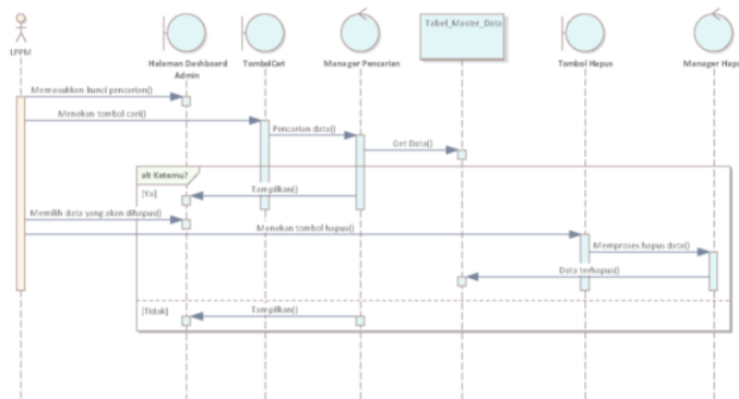
Gambar 13. Sequence Diagram Hapus Data
