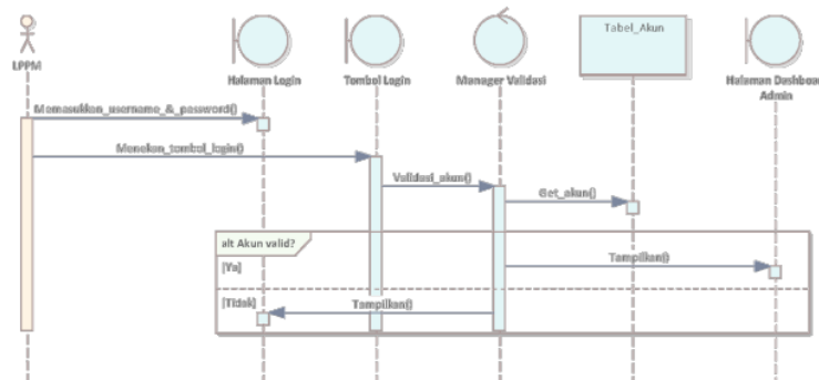
Gambar 9. Sequence Diagram Login
