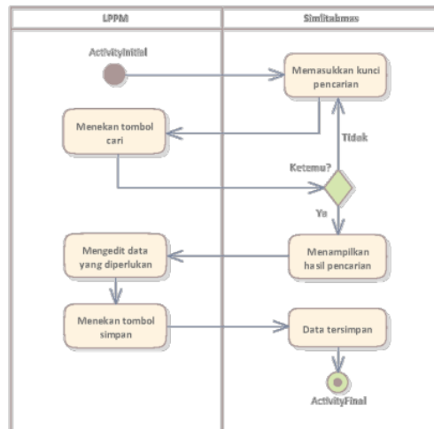
Gambar 6. Activity Diagram Edit Data
