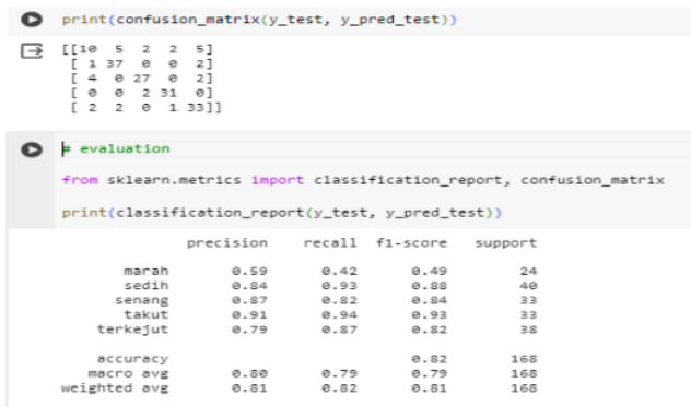
Gambar 2. Confusion Matrix dan Classification Report
