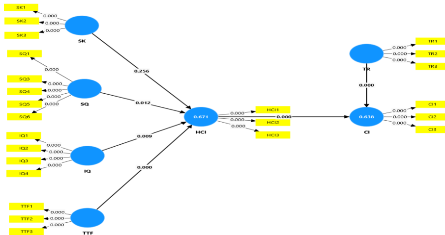
Gambar 1. Hasil bootstrapping
