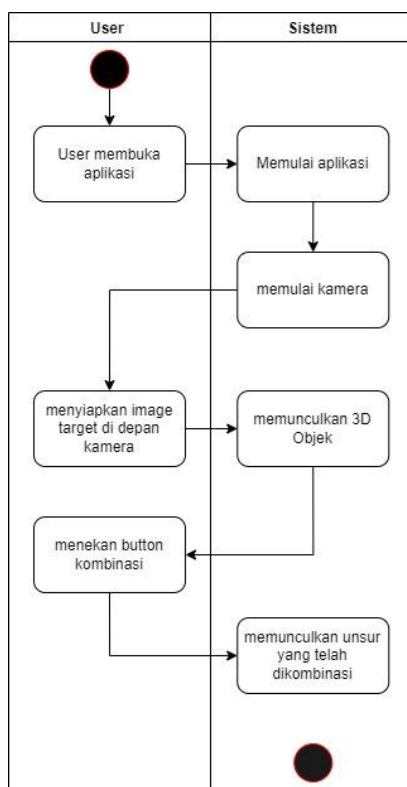
Gambar 4.4 Activity Diagram
