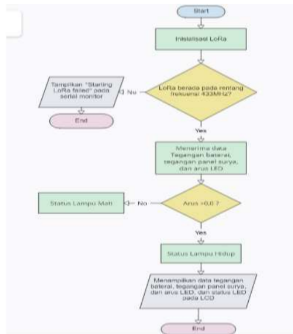
Gambar 4. Flowchart Receiver
