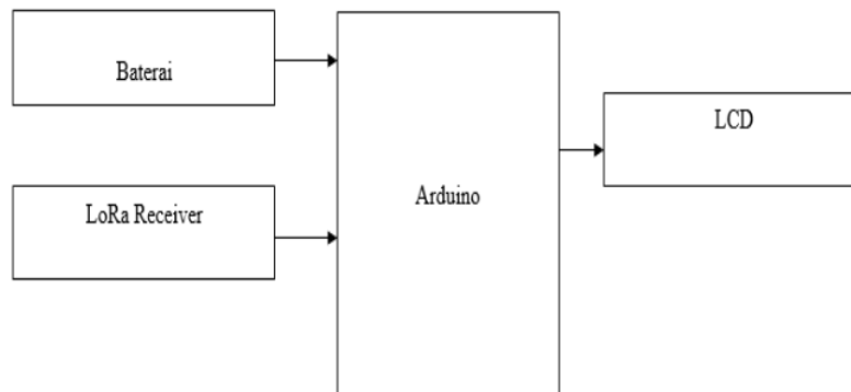
Gambar 2. Diagram Blok Receiver
