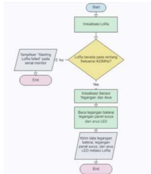
Gambar 3. Flowchart Transmitter
