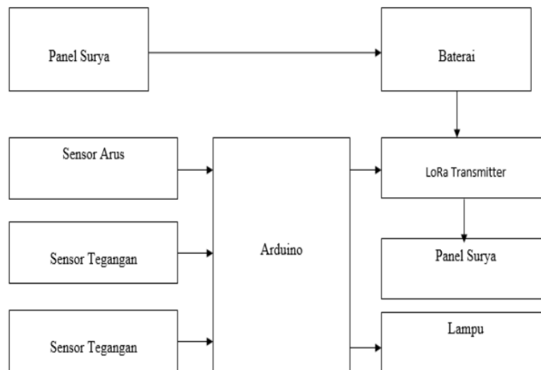
Gambar 1. Diagram Blok Transmitter
