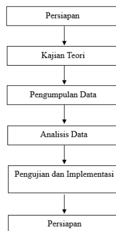
Gambar 1 Metode penelitian
