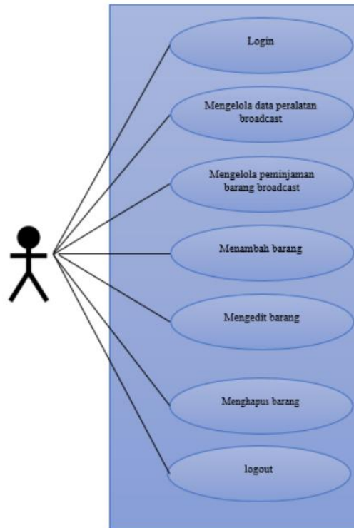
Gambar 3 Use Case Diagram Inventaris Peralatan Broadcast
