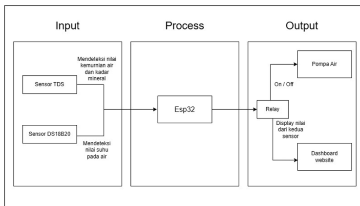
Gambar 2. Blok Diagram
