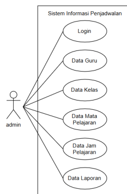
Gambar 1. Use Case Diagram.
