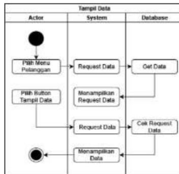
Gambar 9. Activity Diagram Proses Tampil Data
