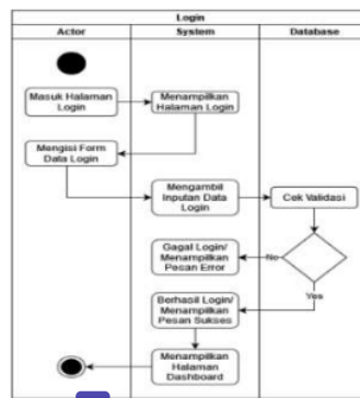
Gambar 7. Activity Diagram Proses Login
