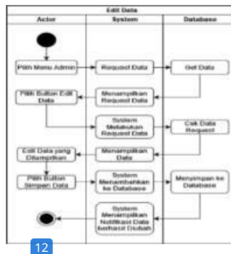
Gambar 10. Activity Diagram Proses Ubah Data
