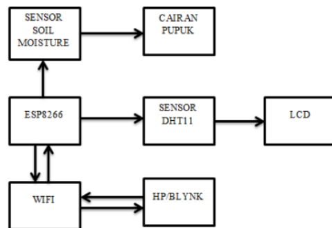
GAMBAR III.2 DIAGRAM BLOK
