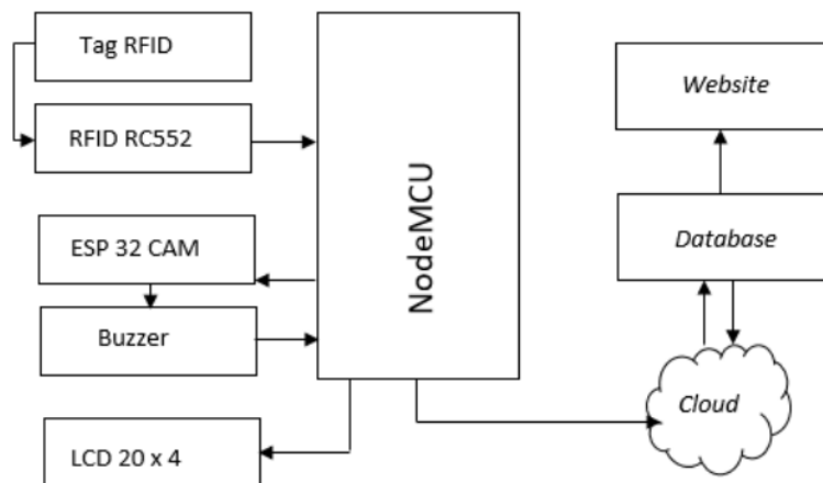
Gambar 6. Blok Diagram
