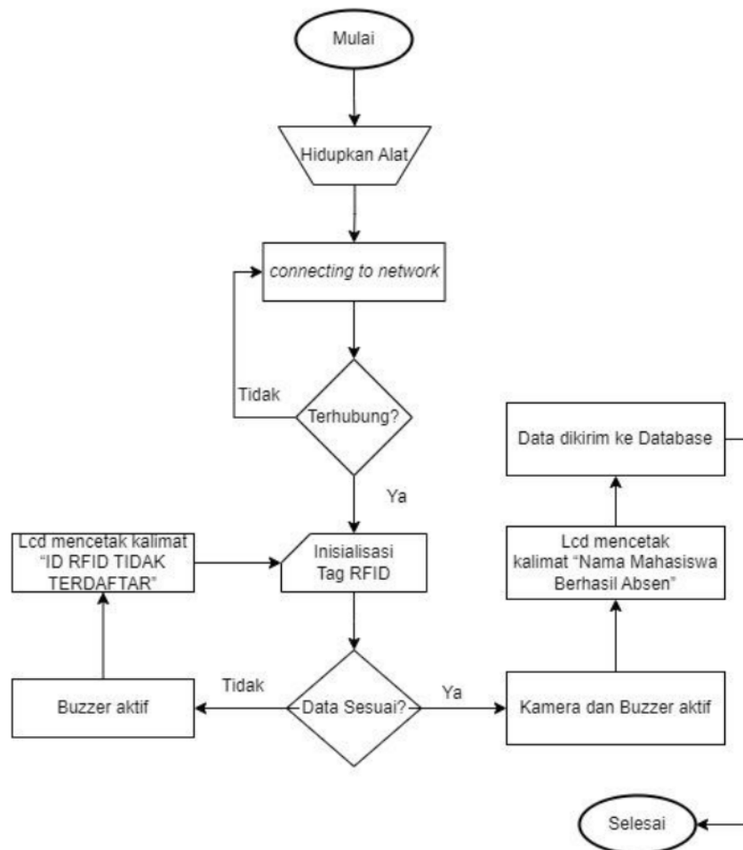
Gambar 5. Flowchart
