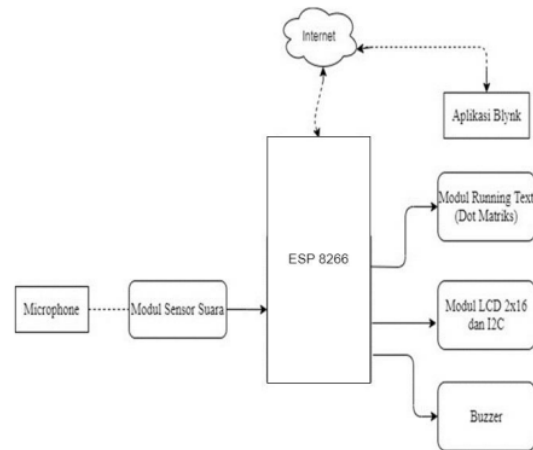
Gambar 7. Blok Diagram
