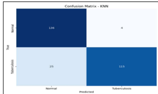
Gambar 7. Confusion matrix Skenario Penelitian 2
