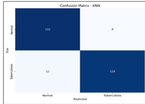
Gambar 5. Confusion matrix Skenario Penelitian 1
