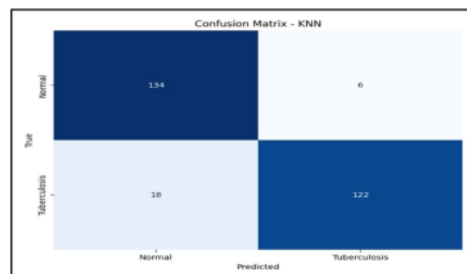
Gambar 9. Confusion matrix Skenario Penelitian 3
