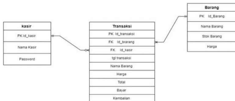
Gambar 4. Diagram
