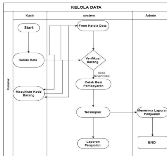
Gambar 3. Activity Diagram
