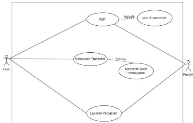
Gambar 2. Use case
