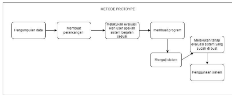
Gambar 1 metode Prototype
