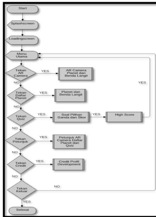
Gambar 2. Flowchart Diagram Augmented Reality
