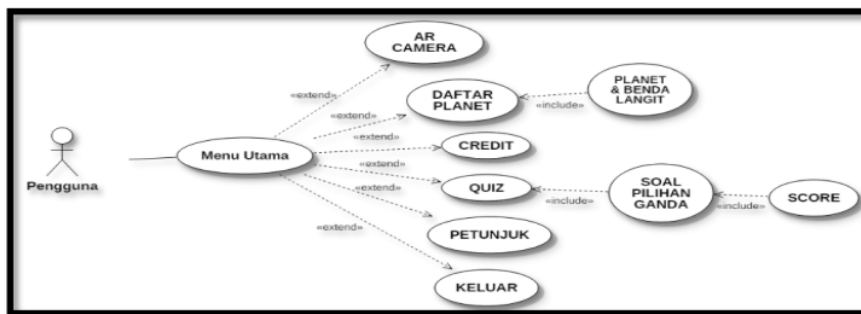
Gambar 3. Use Case Diagram Augmented Reality
