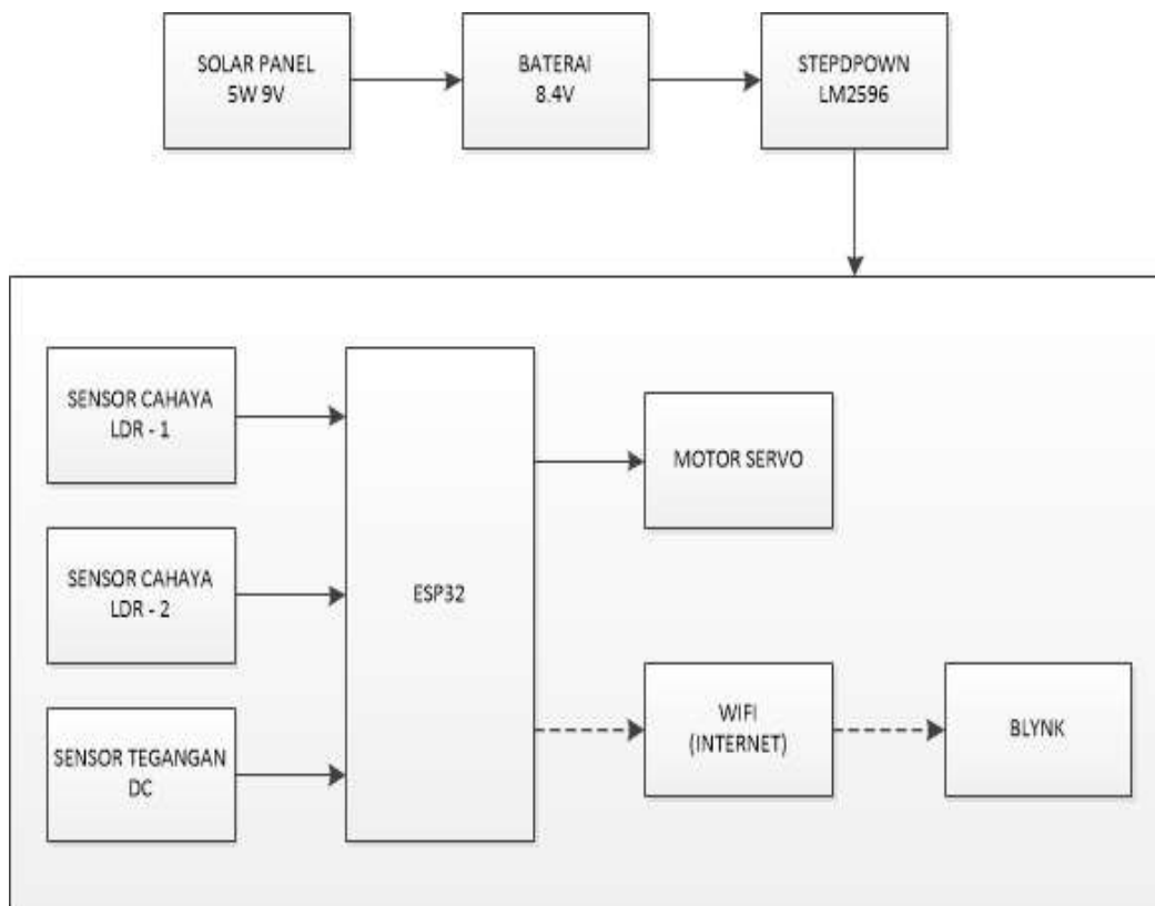
Gambar 7. Blok Diagram
