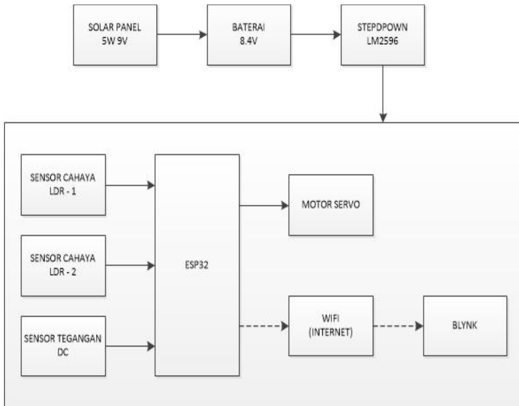
Gambar 7. Blok Diagram
