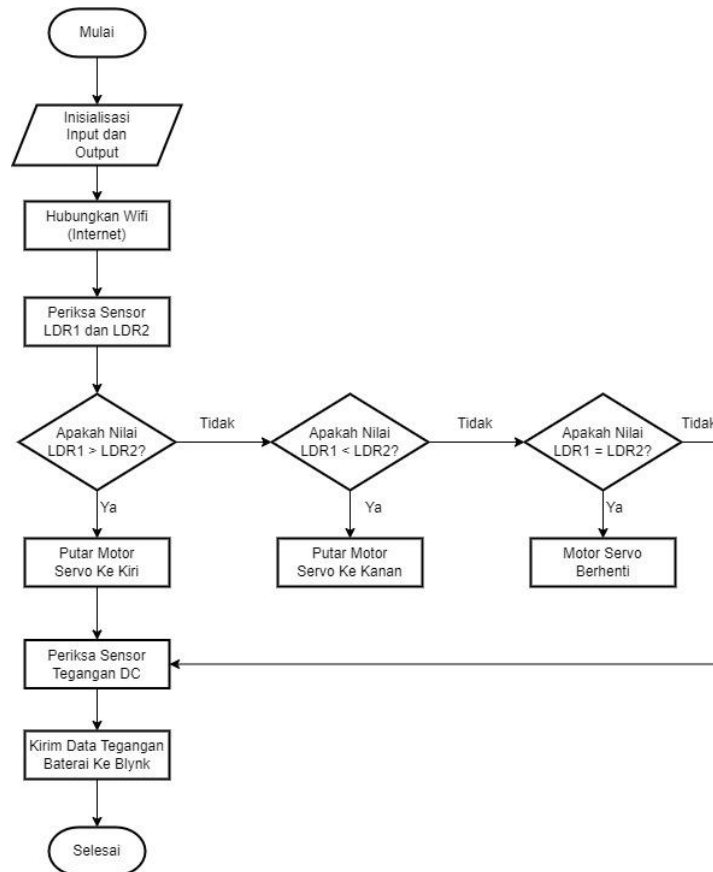
Gambar 6. Flowchart
