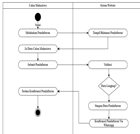
Gambar 4. Activity Diagram Pendaftaran
