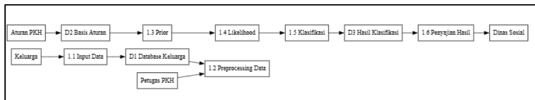
Gambar 3. DFD Level 1.
