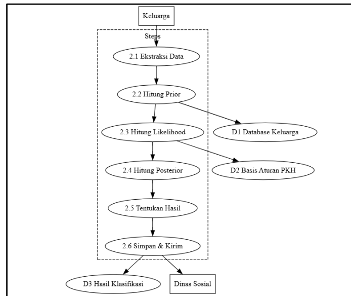
Gambar 4. DFD Level 2.
