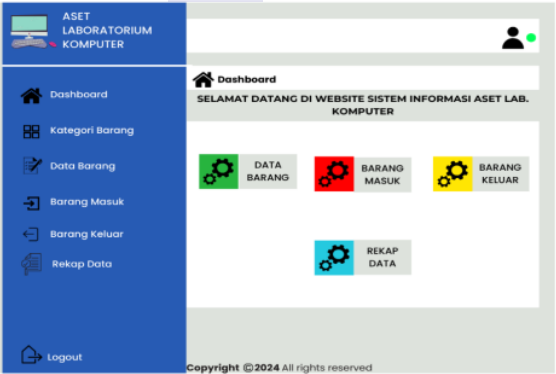
Gambar 6. Halaman Dashboard
