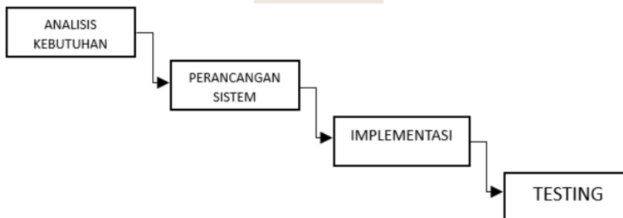
Gambar 1. Metode Waterfall
