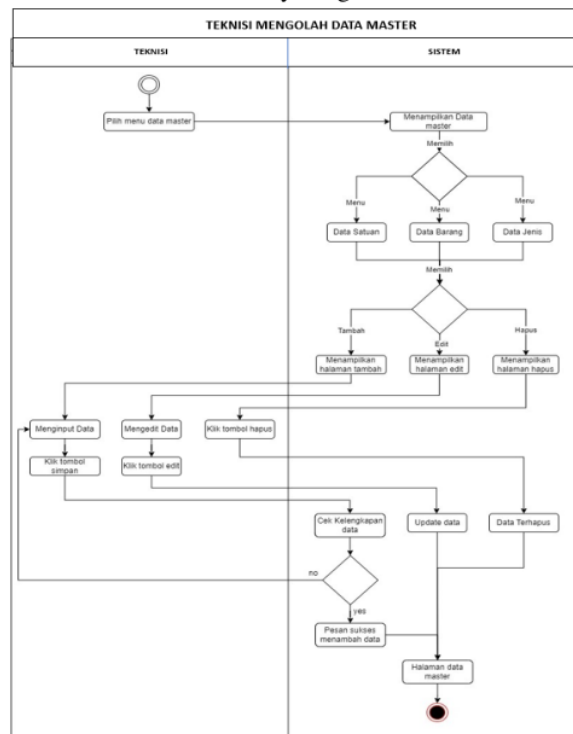
Gambar 3. Activity Diagram
