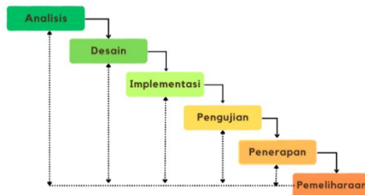
Gambar 1 Diagram Waterfall
