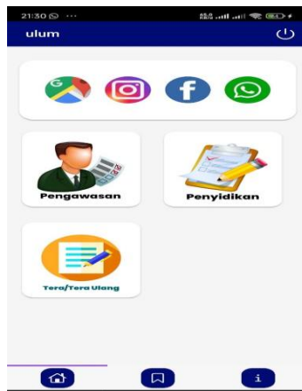
Gambar 7 Halaman Dashboard
