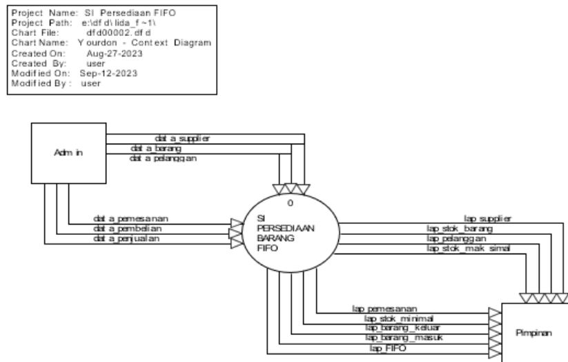
Gambar 3.3 Context Diagram
