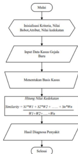
Gambar 1. Flowchart Algoritma Case Base Reasoning (CBR)
