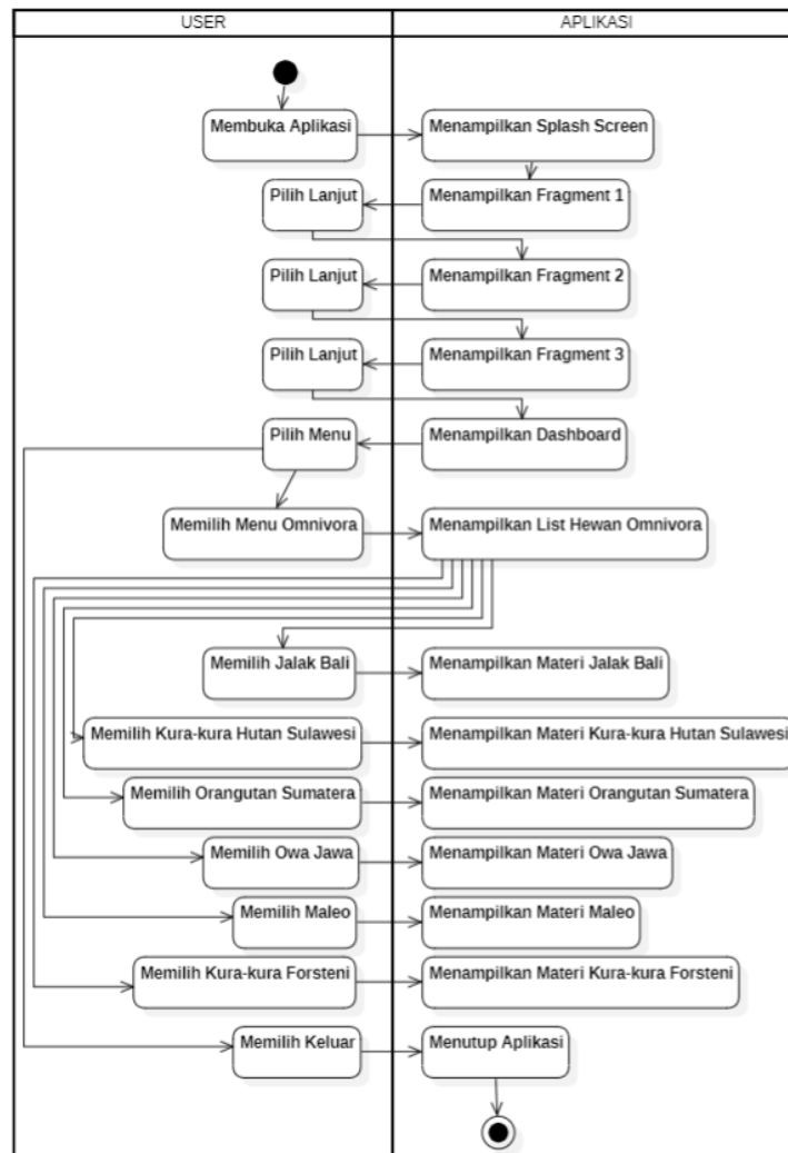
Gambar 7 Activity Diagram Omnivora
