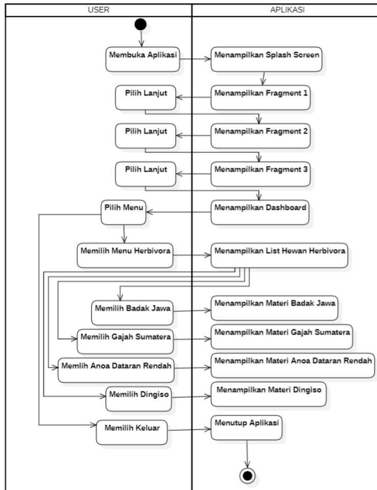
Gambar 4. Activity Diagram Herbivora
