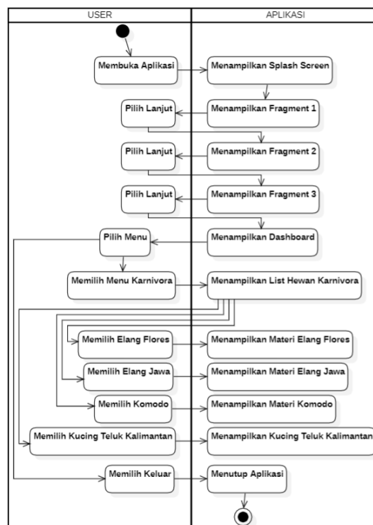
Gambar 6 Activity Diagram Karnivora
