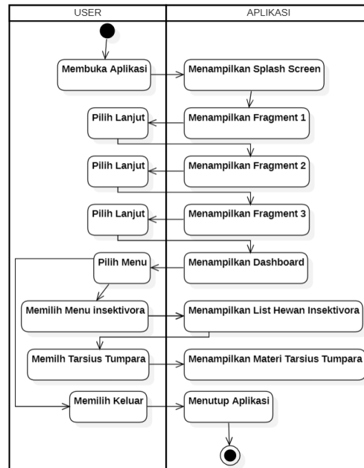
Gambar 5 Activity Diagram Insektivora
