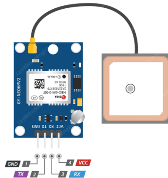
Gambar 3. GPS Neo-6L
