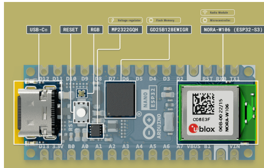
Gambar 1. ESP32 Micro Controller
