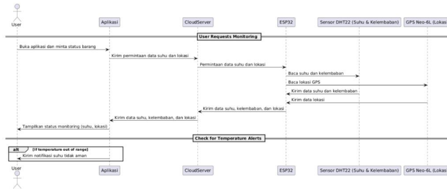
Gambar 5. Sequence Diagram
