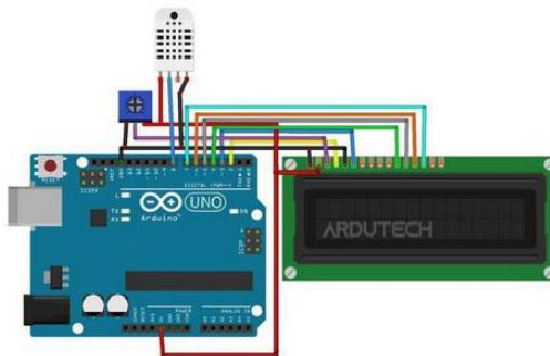
Gambar 2. Rangkaian Sensor Suhu DHT22
